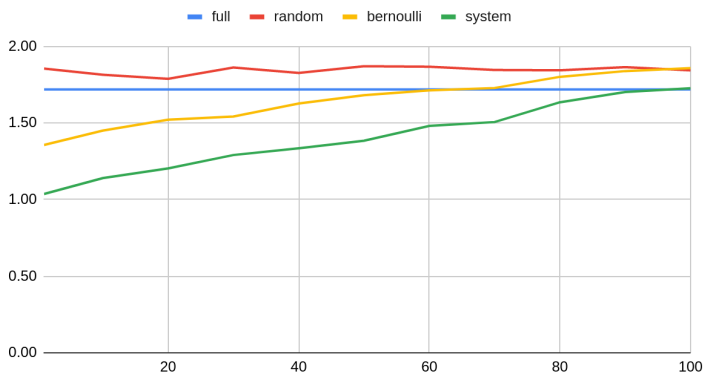
sampling performance / 10k rows / local
