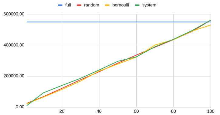
sampling performance / 100M rows / remote (192.168.0.164)
