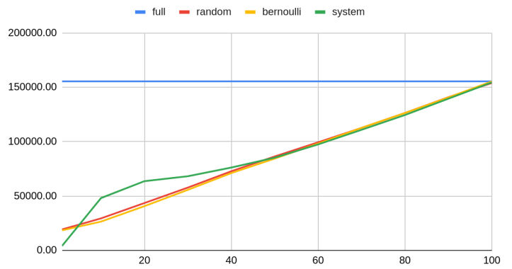
sampling performance / 100M rows / fdw (127.0.0.1)
