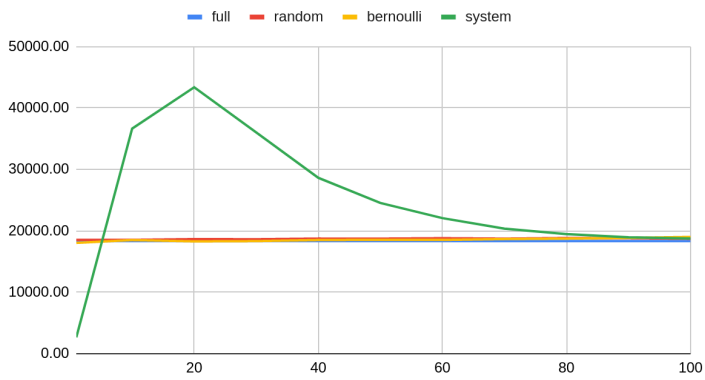
sampling performance / 100M rows / local
