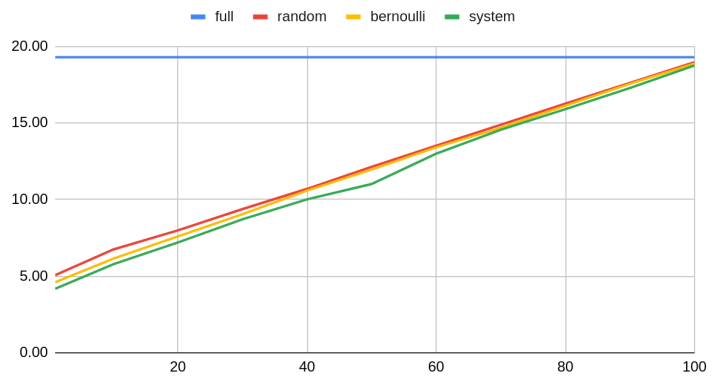
sampling performance / 10k rows / fdw (127.0.0.1)
