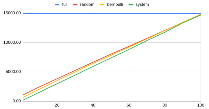
sampling performance / 10M rows / fdw (127.0.0.1)
