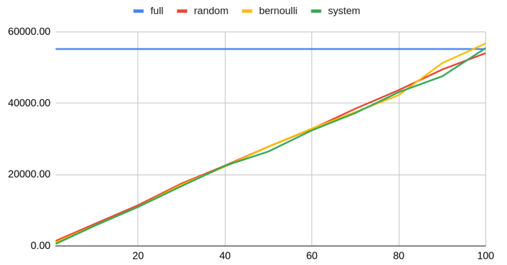
sampling performance / 10M rows / remote (192.168.0.164)
