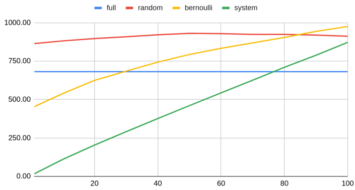
sampling performance / 10M rows / local
